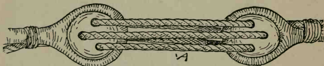
FIG. 98.—Deadeye lashing.
